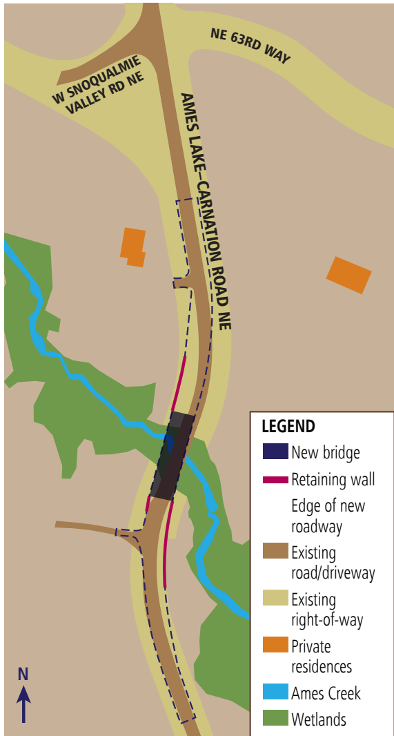
The new bridge will straighten out the roadway to increase sight-lines and safety.
